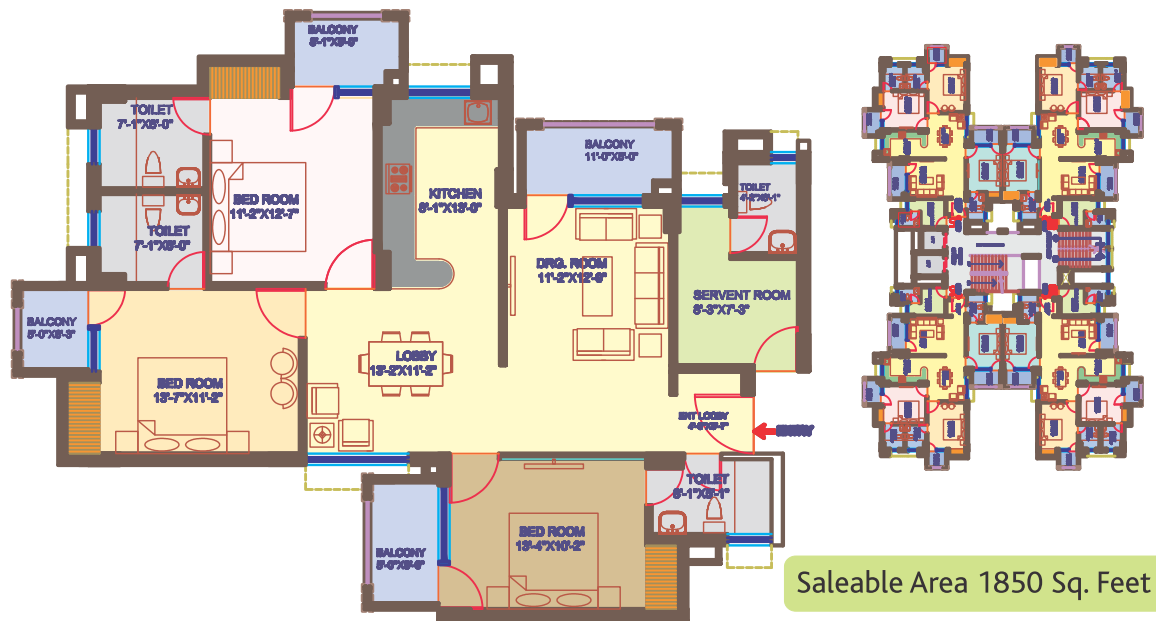
TYPICAL FLOOR PLAN TOWER-D, SRS RESIDENCY, SECTOR-88, FARIDABAD
